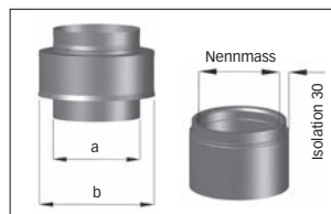
Typ 1 Dila/Stulpring Isolation 30 mm
